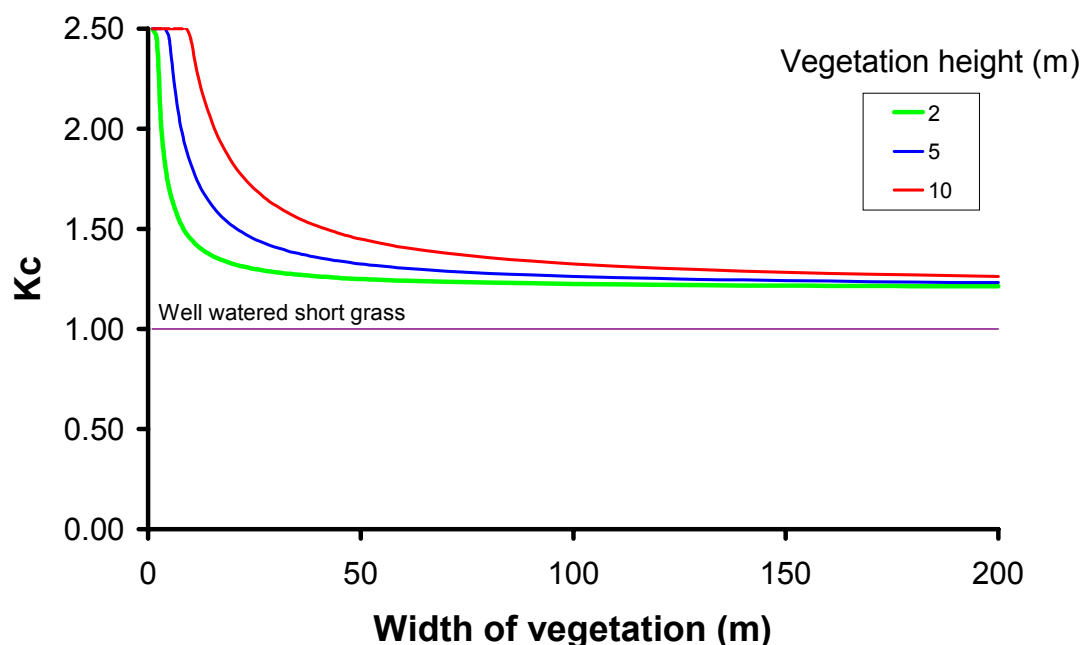
Figure 4). A strip of vegetation 10 m high and 50 m wide might transpire 45% more than a similar width of short grass. Though the effect decreases rapidly, it is still noticeable even for vegetation widths of 200 m. The implications for design of coppice planting in sensitive areas could be significant and suggests that narrow strips of coppice planted across the prevailing wind direction should not be recommended.
