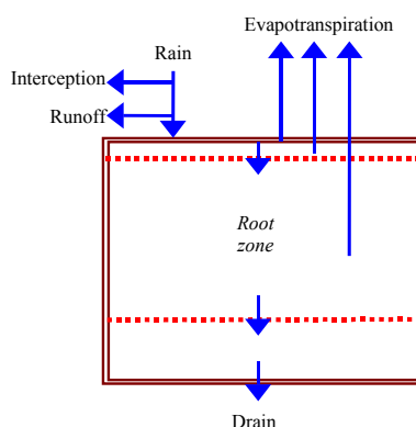
Figure 5. Schematic representation of the WaSim soil water balance model
