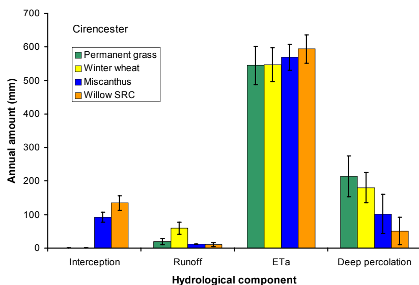
Figure 6. Comparison of simulated interception, annual runoff, evapotranspiration and deep percolation for permanent grass, winter wheat, Miscanthus and willow SRC grown on sandy clay loam soil at Silsoe, Beds (1970 – 1999), Selby, Yorks (1970 – 1999) and at Cirencester, Wilts (1983 – 1999).
