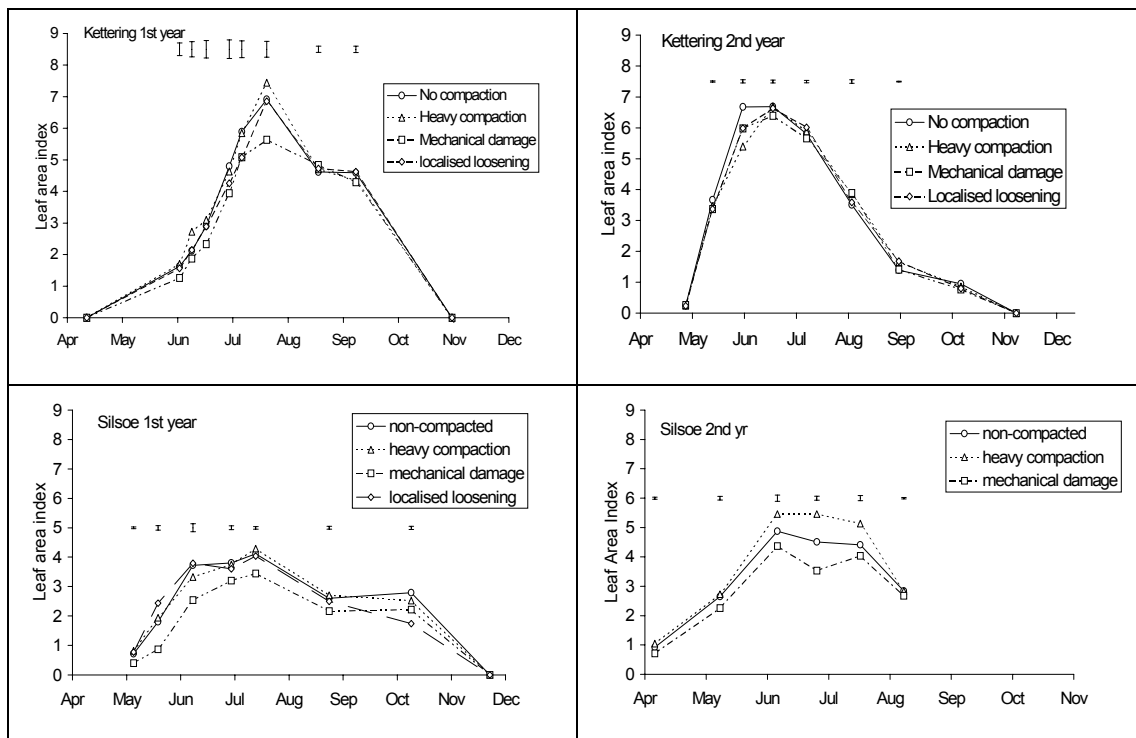
Figure 2. The effect of harvesting damage on leaf area index development of Salix viminalis cv Q683 in the first year of growth after harvesting at Kettering (top) and Silsoe (bottom) and in the first (left hand side) and second (right hand side) years of growth after harvesting. Error bars are the standard error of the difference between means, n = 30 (Souch et al. , 2000a).
