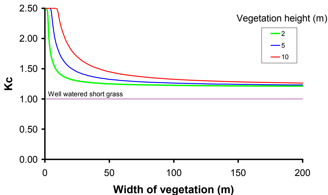
Figure 4. The theoretical effect of vegetation height and width on crop coefficient ( K_c ) for conditions where: mean temperature = 22 °C; bulk stomatal resistance = 40 s m -1 ; wind speed = 2 m s -1 . Adapted from Allen et al. (1998).
